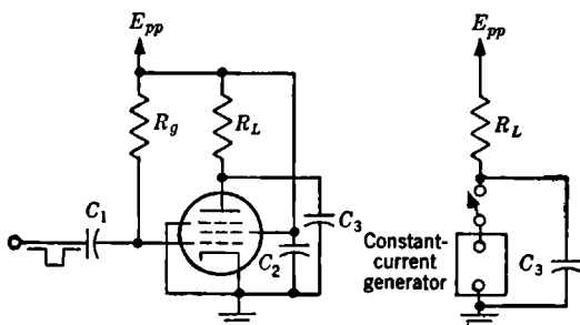
FIG. 4-3.—Equivalent circuit of an overdriven pentode.
